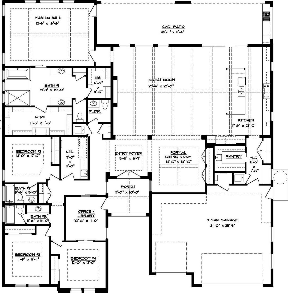
FLOOR PLAN 70'-1" x 75'-1"
