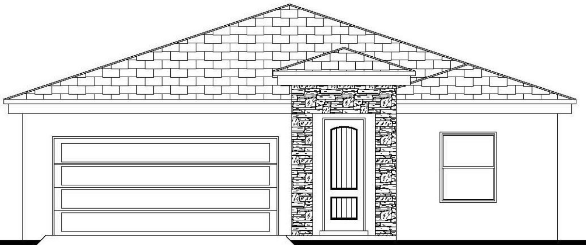
FRONT ELEVATION
