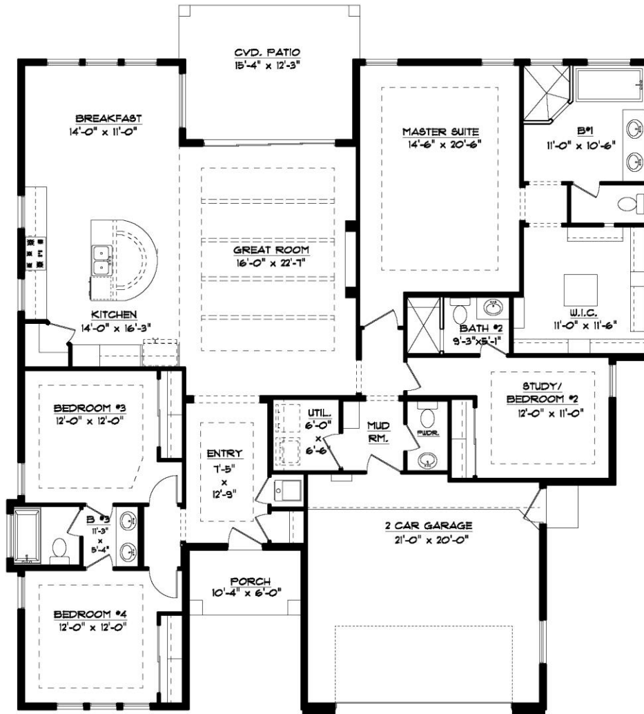
FLOOR PLAN 58'-0" x 58'-7"
