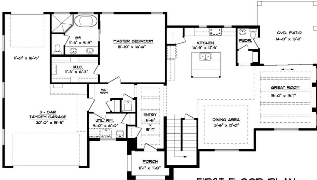
FIRST FLOOR PLAN 75'-8" x 37'-1 1/2"
