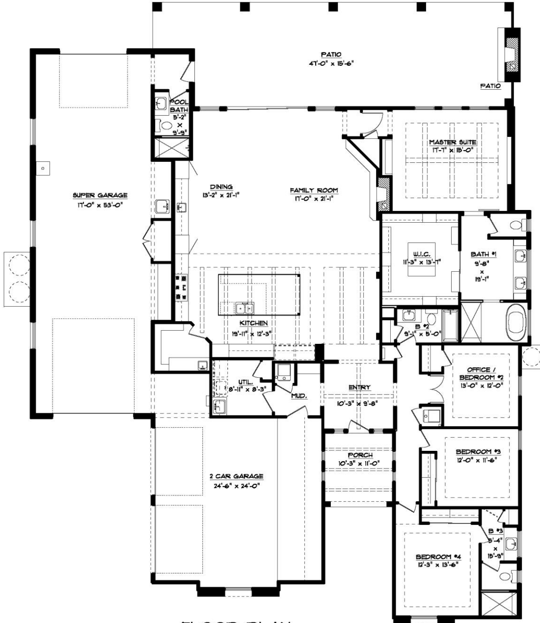
FLOOR PLAN 73'-3 1/2" x 83'-8 1/2"
