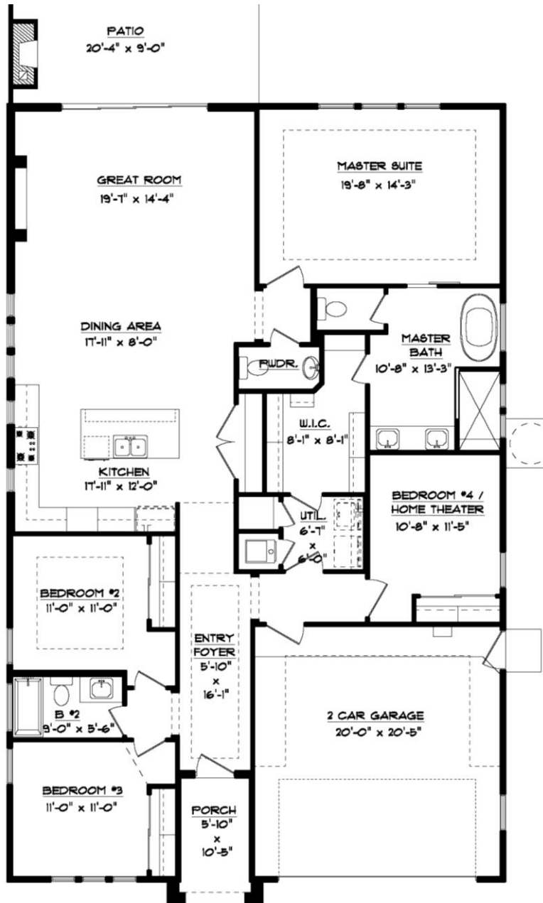
FLOOR PLAN 40'-3 1/2" X 63'-2"
