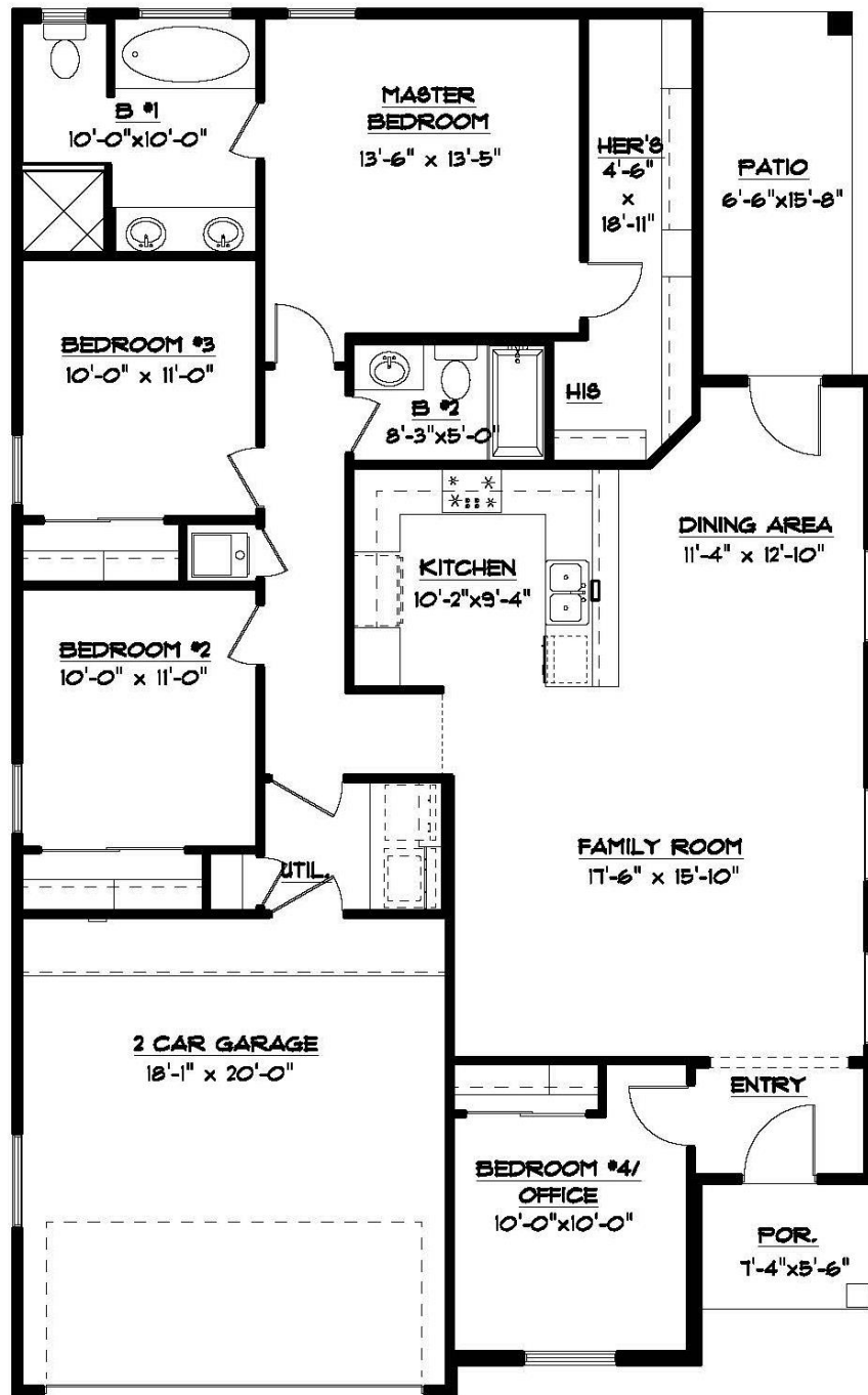
FLOOR PLAN 36'-6" x 59'-0"
