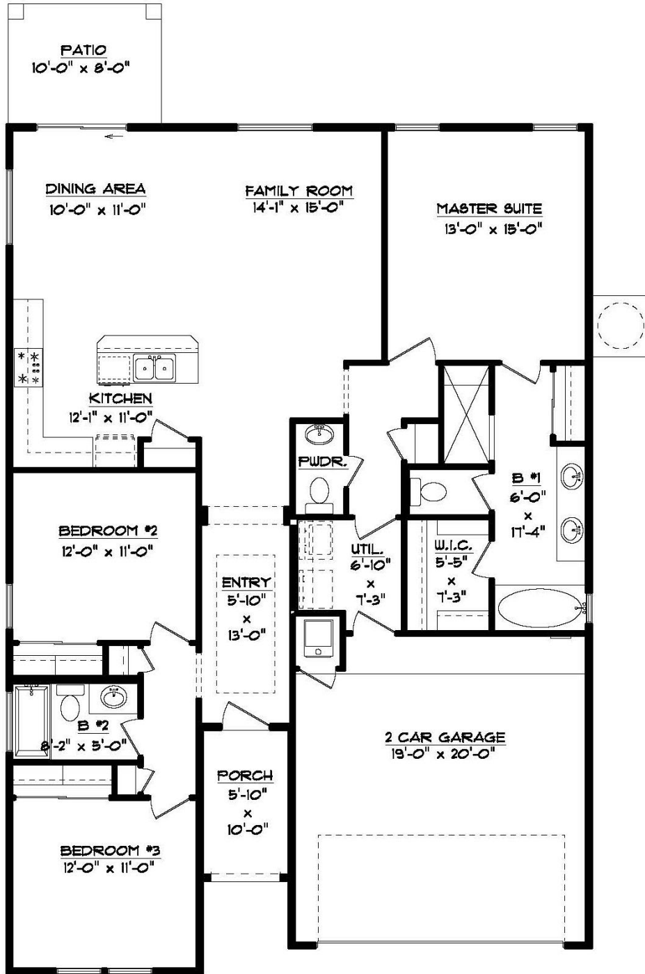
FLOOR PLAN 38'-0" x 55'-3"
