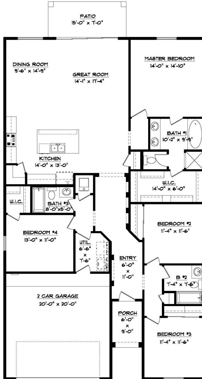
FLOOR PLAN 38'-6" x 65'-6"
