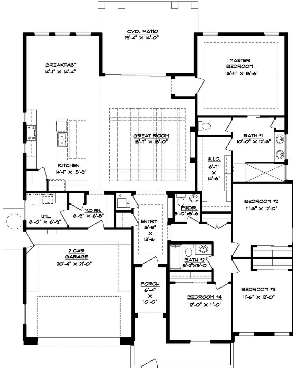
FLOOR PLAN 52'-4" x 59'-11"
