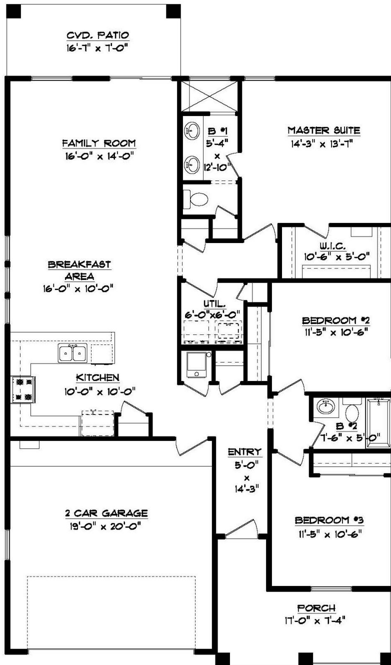
FLOOR PLAN 36'-11 1/2" x 54'-10 1/2"
