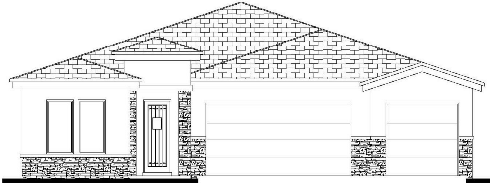
FRONT ELEVATION - S
