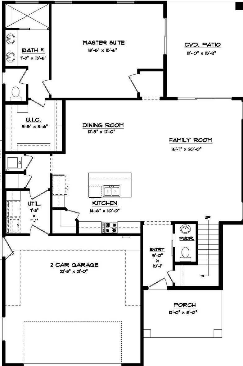
FIRST FLOOR PLAN 39'-6" x 59'-8"
