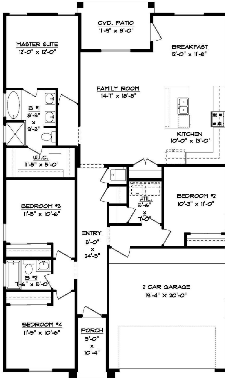
FLOOR PLAN 36'-11 1/2" x 59'-1 1/2"
