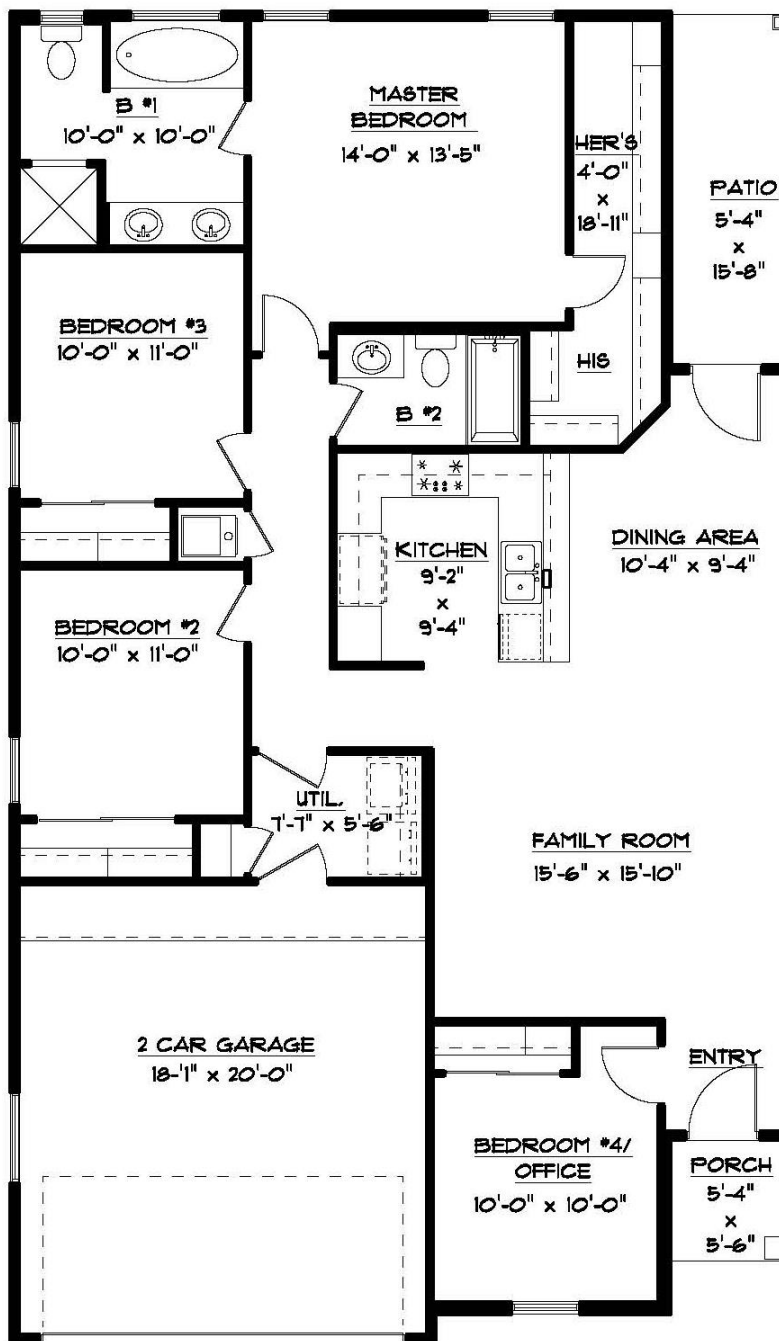
FLOOR PLAN 34'-6" x 59'-0"
