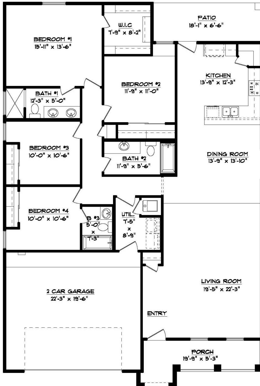
FLOOR PLAN 42'-7 1/2" x 61'-0"
