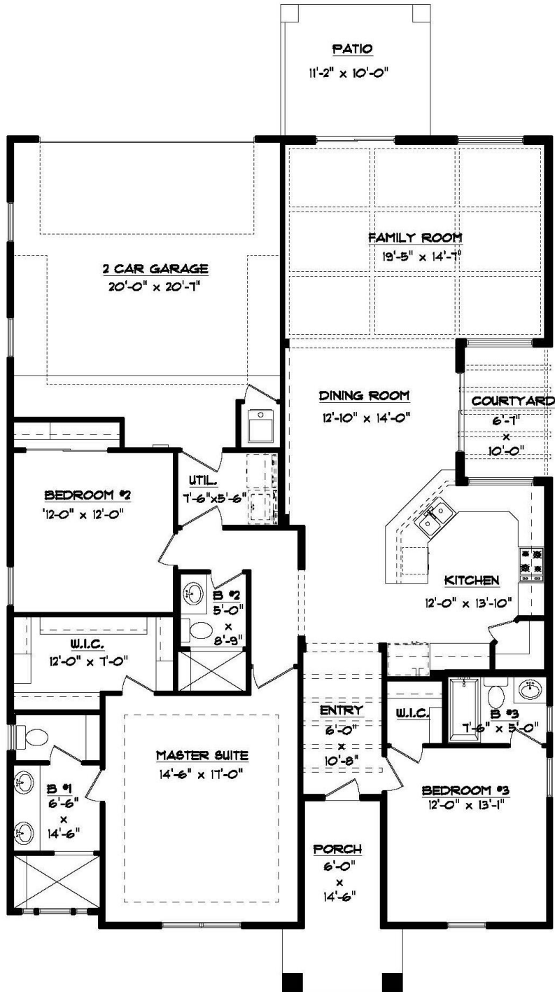
FLOOR PLAN 40'-6" x 58'-11 1/2"
