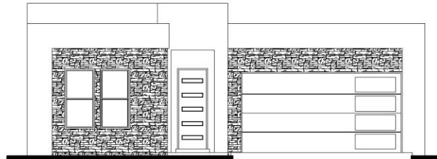
FRONT ELEVATION - C
