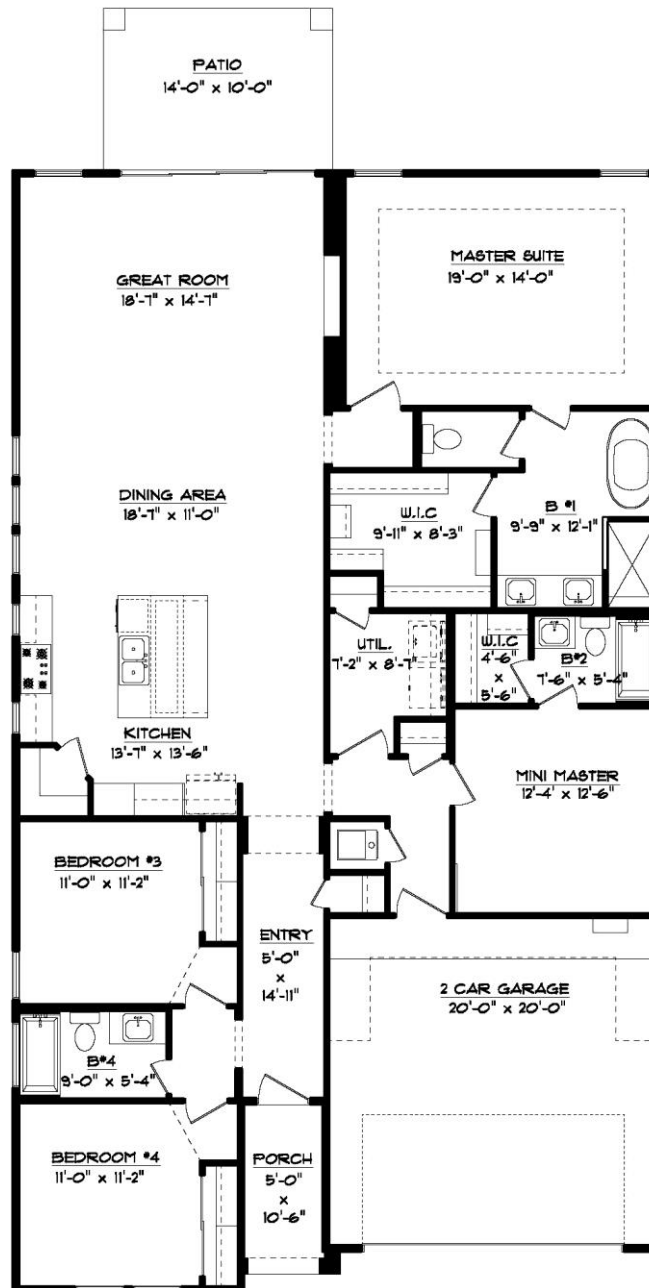
FLOOR PLAN 39'-6" x 68'-4 1/2"
