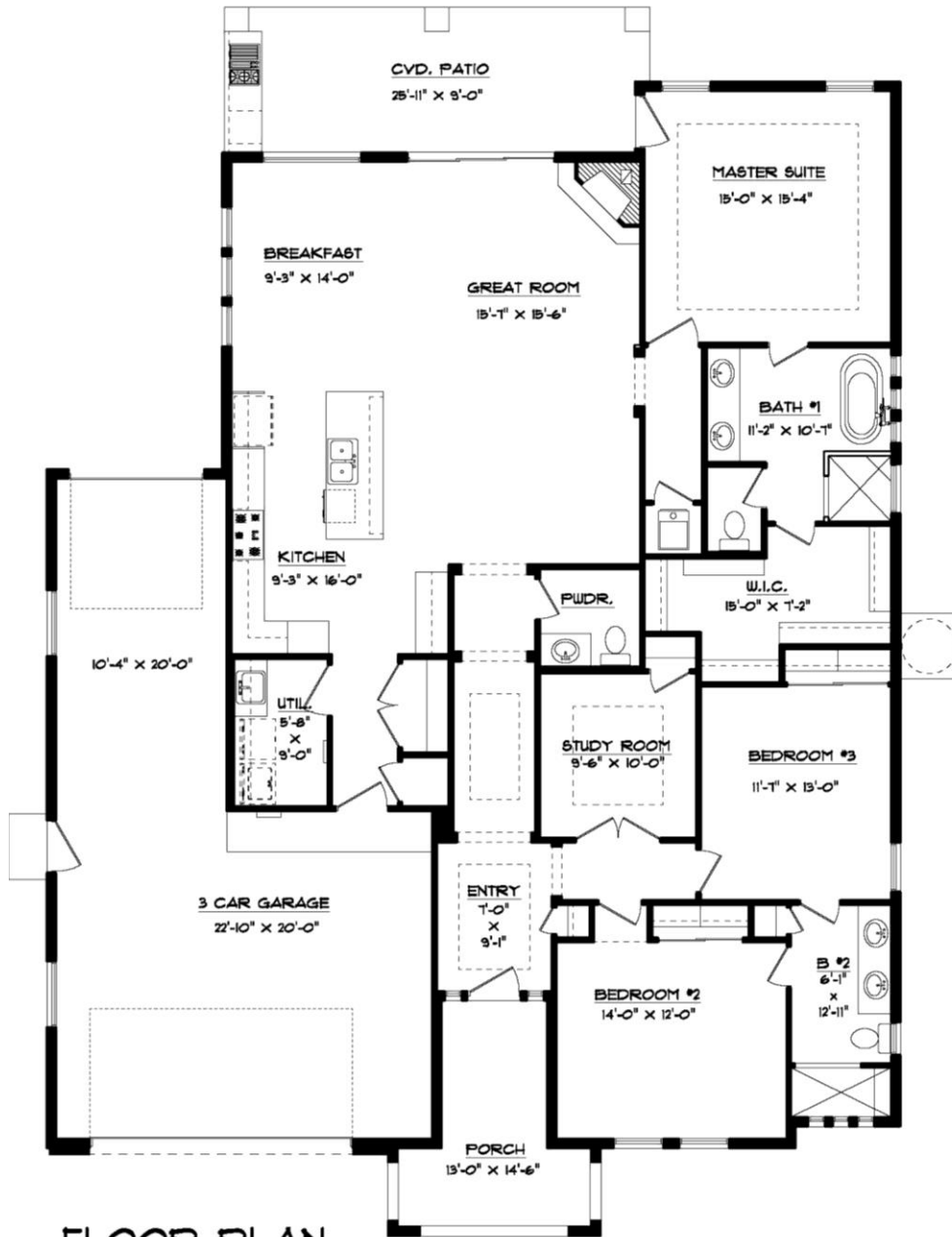
FLOOR PLAN 51'-9" X 64'-10"
