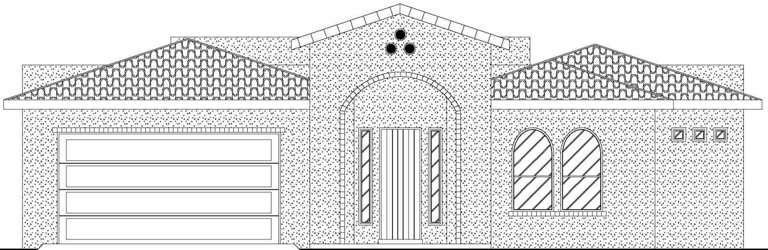
FRONT ELEVATION
