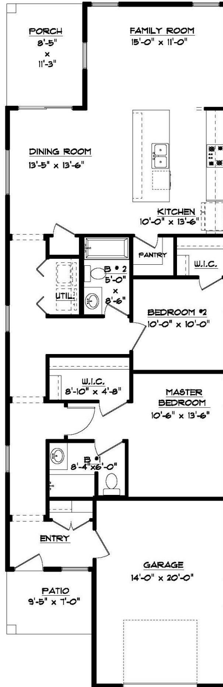
FLOOR PLAN 24'-0" x 74'-3 1/2"
