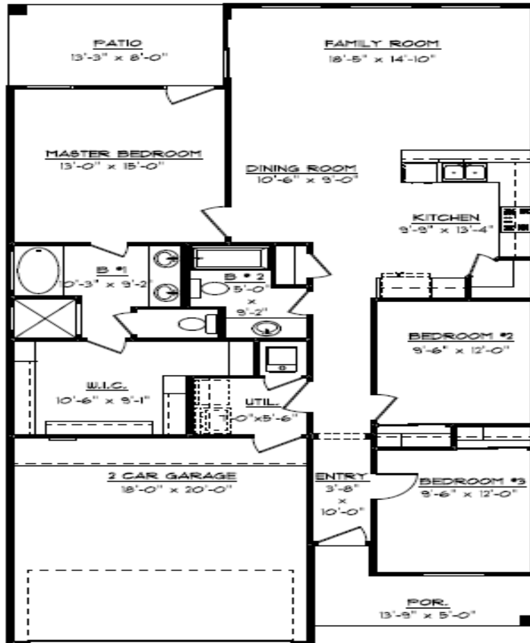
FLOOR PLAN 32'-4" x 62'-9"
