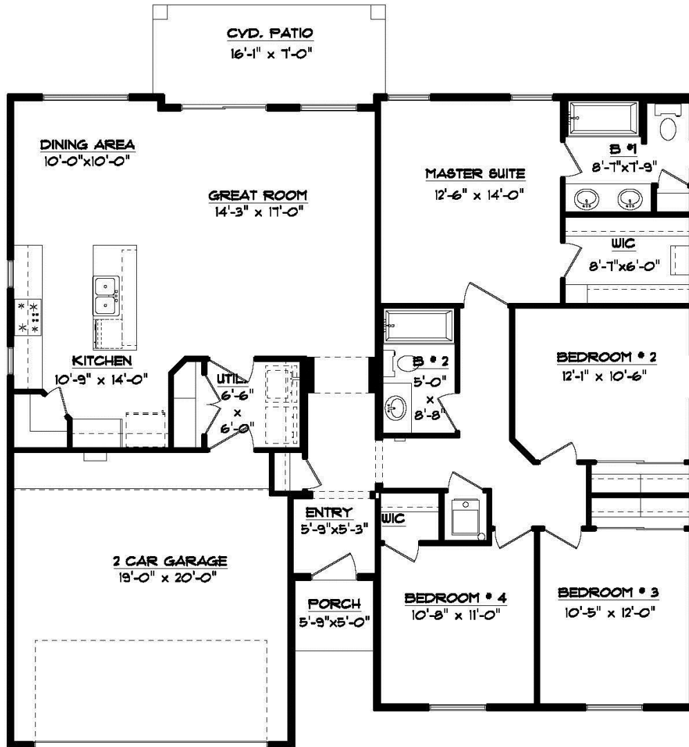
FLOOR PLAN 47'-4" x 44'-10 1/2"
