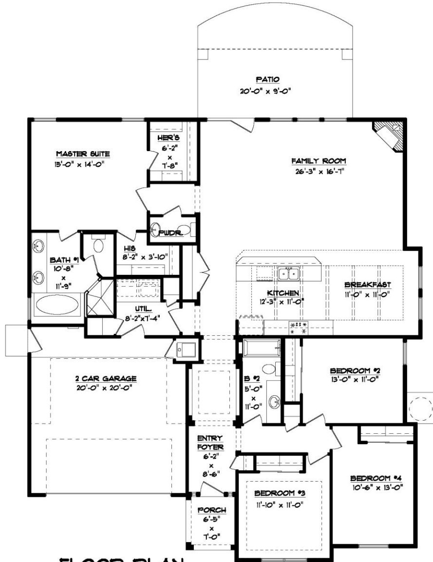
FLOOR PLAN 50'-7 1/2" x 56'-10"
