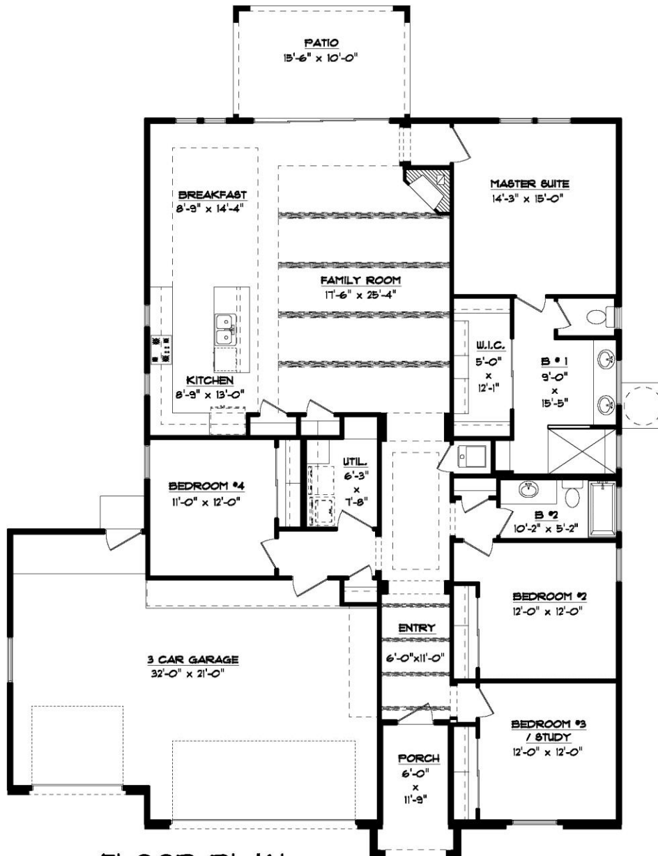
FLOOR PLAN 53'-6" x 61'-6"
