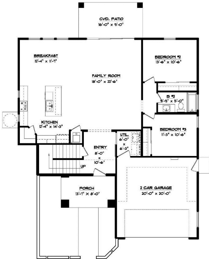
FIRST FLOOR PLAN 44'-10" X 49'-11 1/2"
