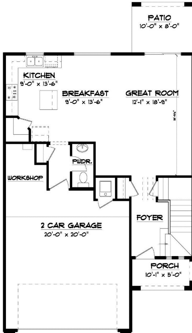
FIRST FLOOR PLAN 30'-8" x 43'-3 1/2"
