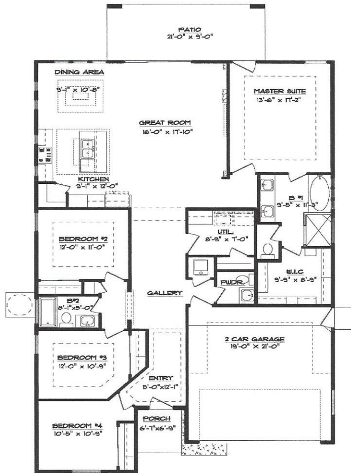
FLOOR PLAN
