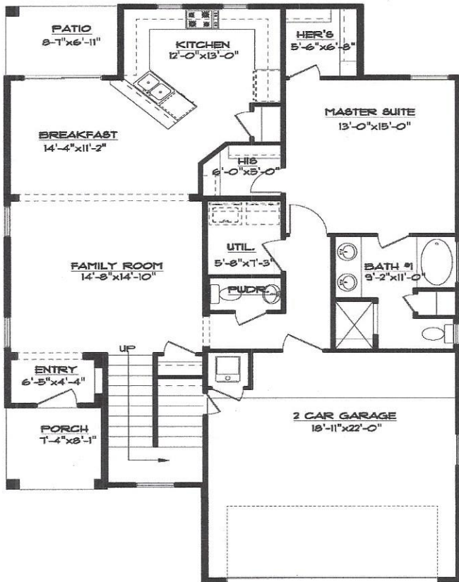
FIRST FLOOR PLAN 34'-6" x 56'-1 1/2"
