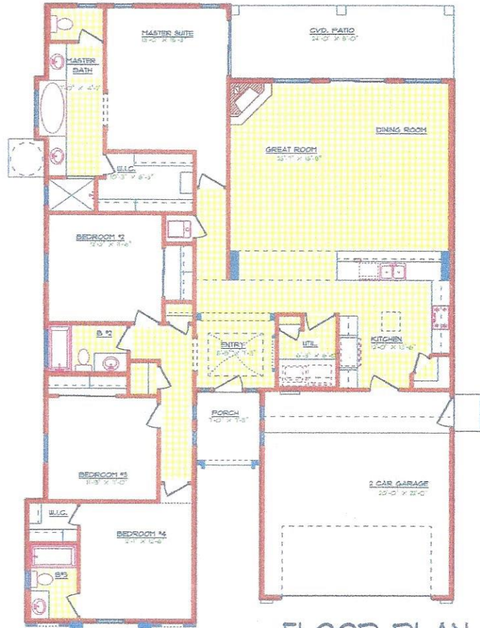
FLOOR PLAN
