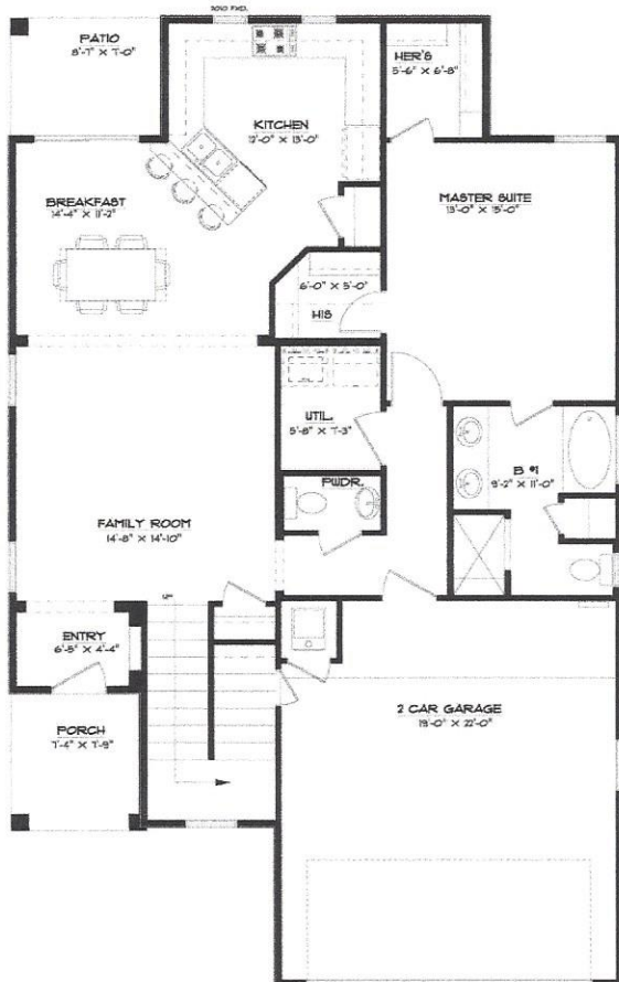
FIRST FLOOR PLAN W 34'-6" X D 56'-1 1/2"
