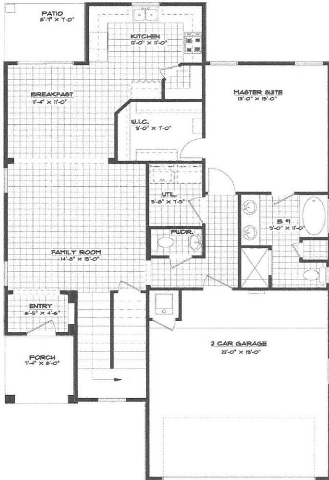
FIRST FLOOR PLAN W 34'-6" X D 56'-2"
