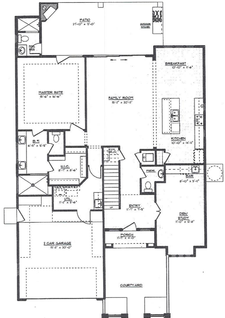
FIRST FLOOR PLAN 43'-0" x 64'-7"
