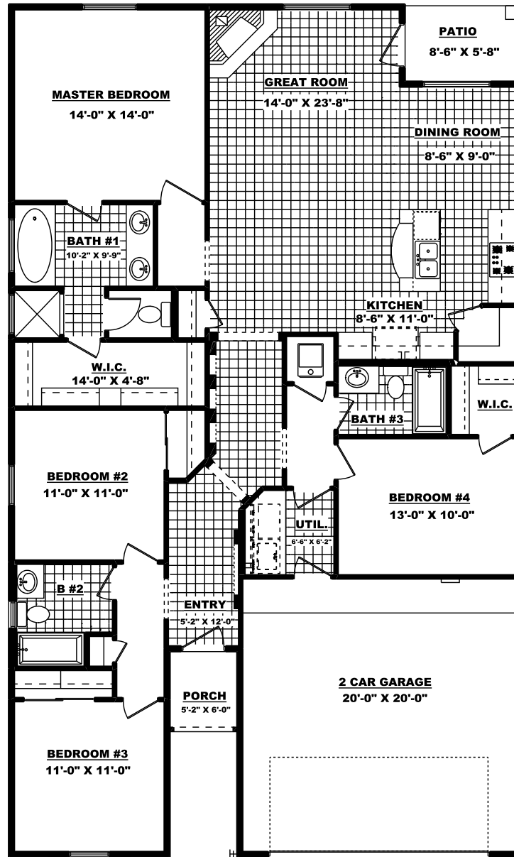
FLOOR PLAN
