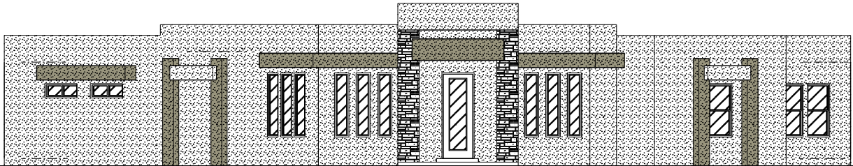
FRONT ELEVATION
