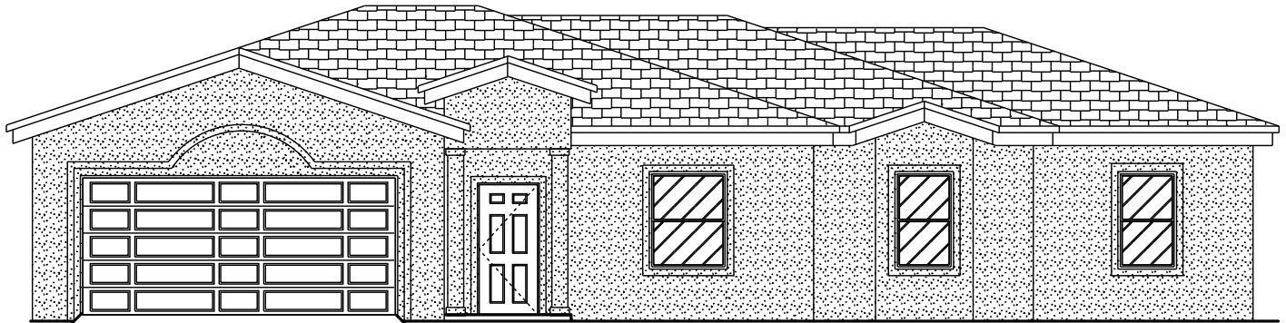
FRONT ELEVATION
