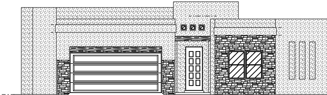
FRONT ELEVATION
