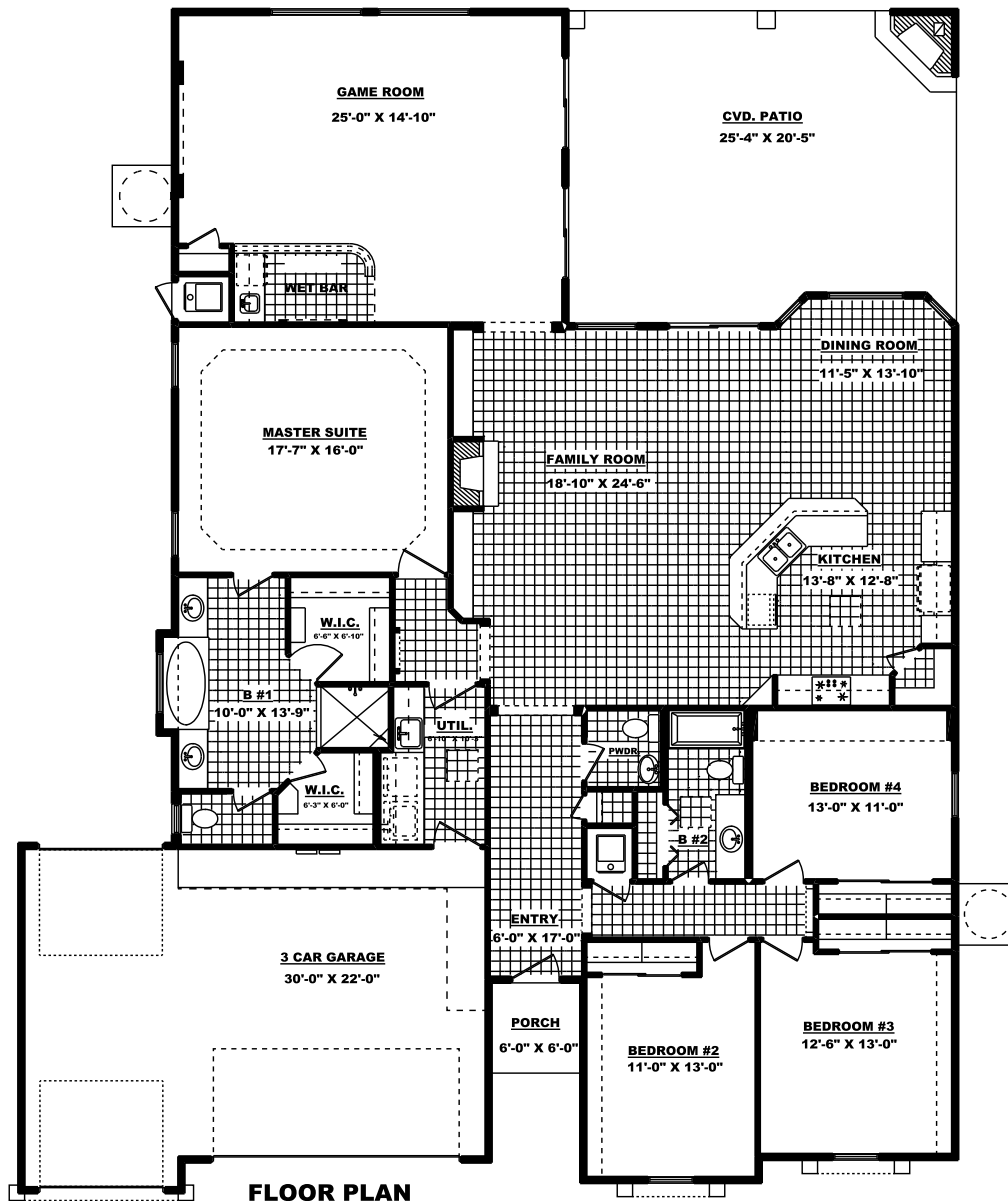
FLOOR PLAN
