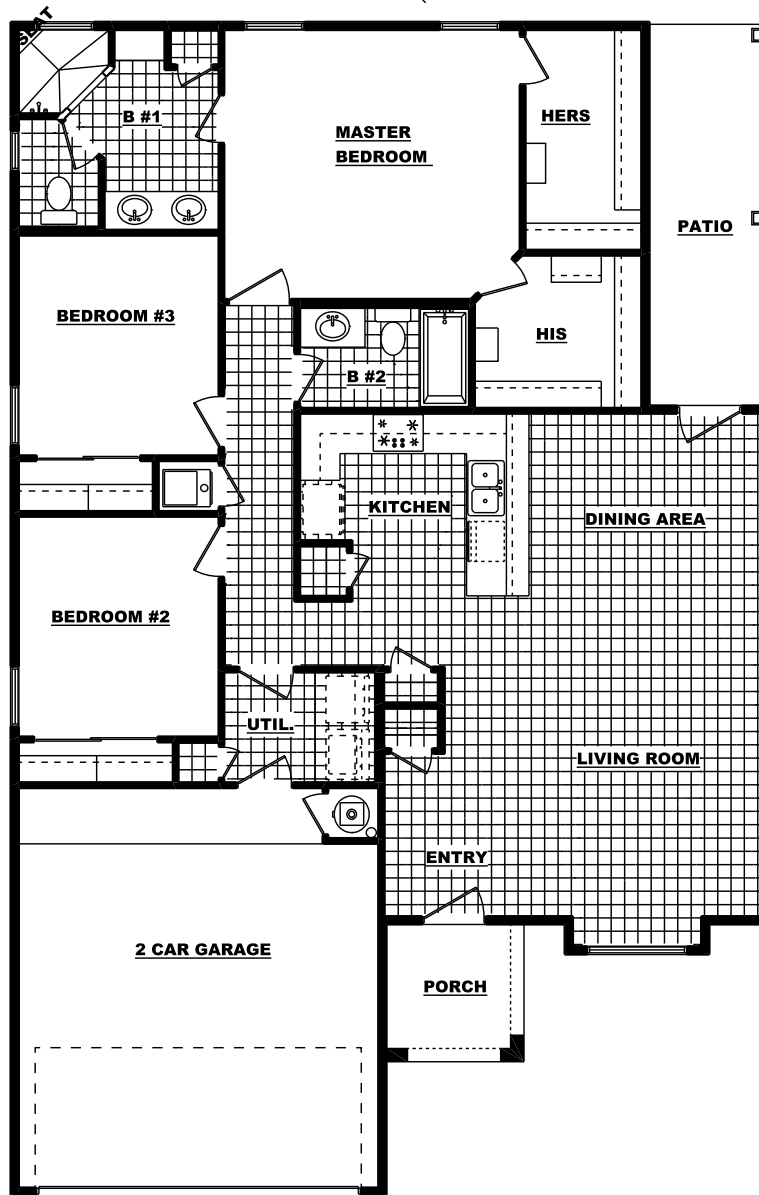
FLOOR PLAN
