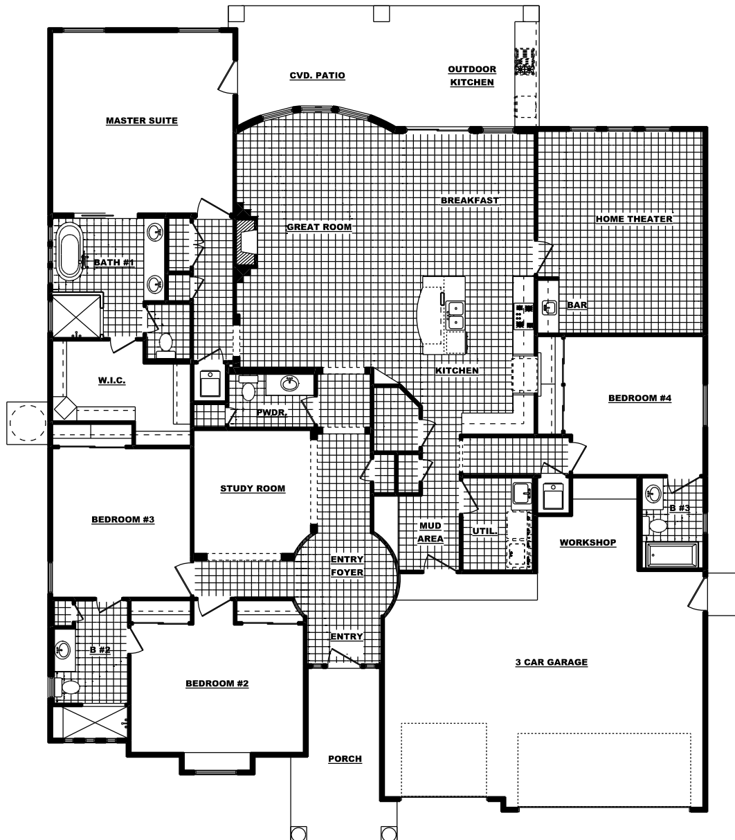
TILE FLOOR PLAN
