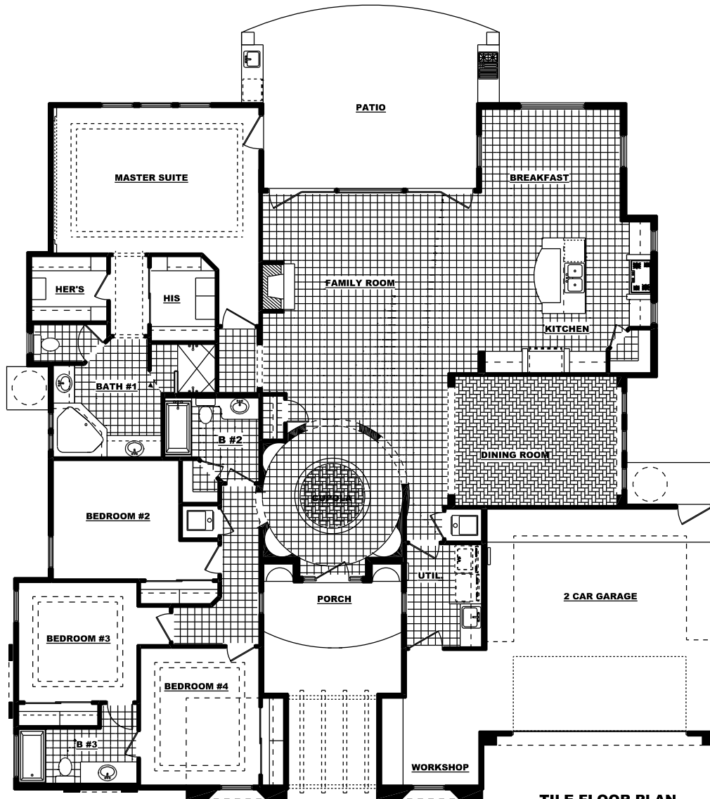
TILE FLOOR PLAN
