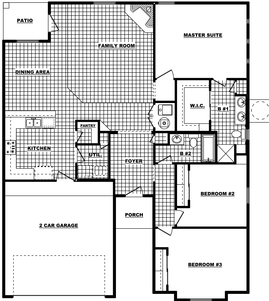
FLOOR PLAN
