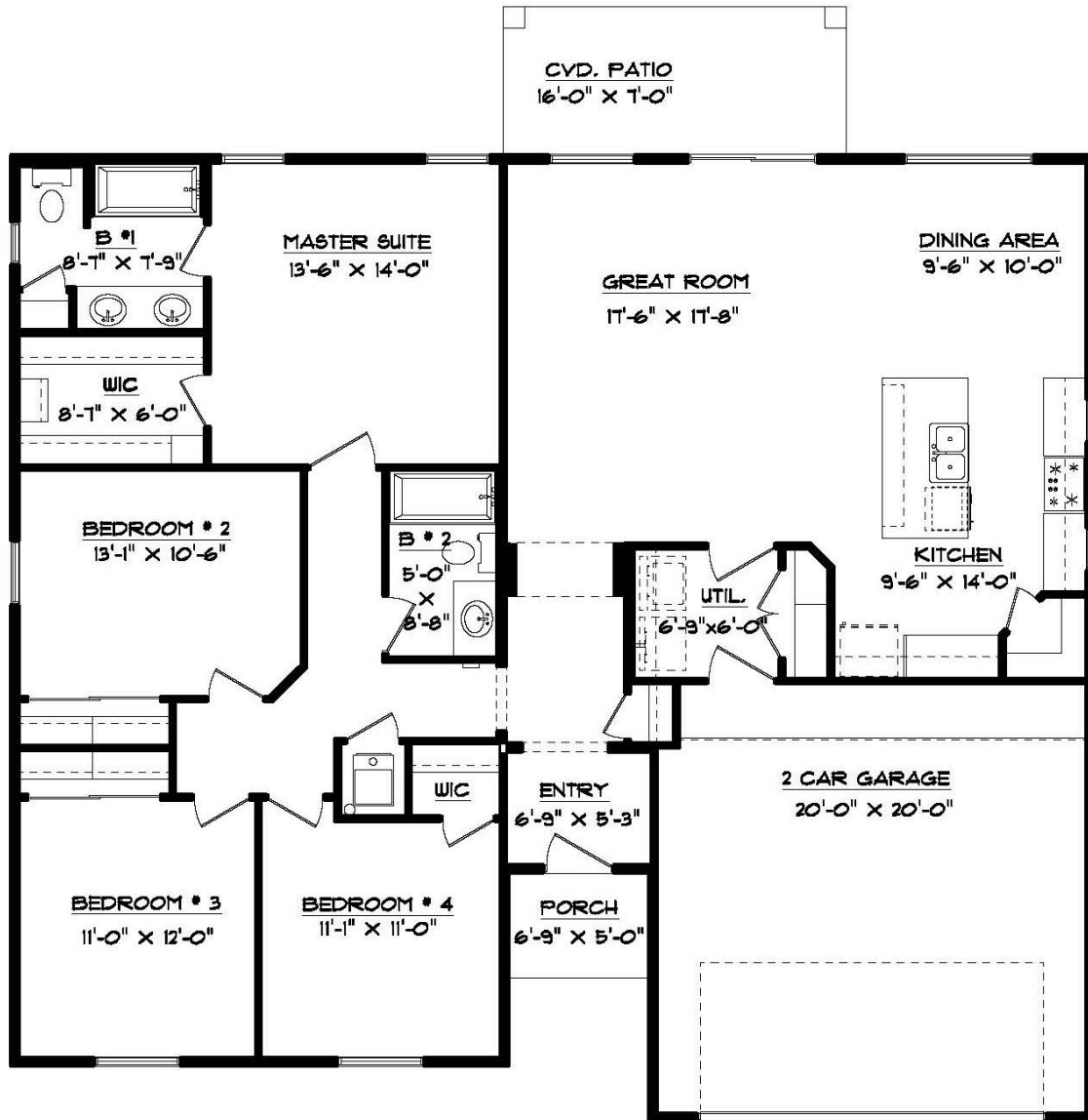
FLOOR PLAN 50'-4" X 44'-10 1/2"
