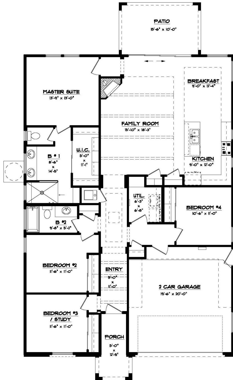
FLOOR PLAN 39'-6" x 56'-6"
