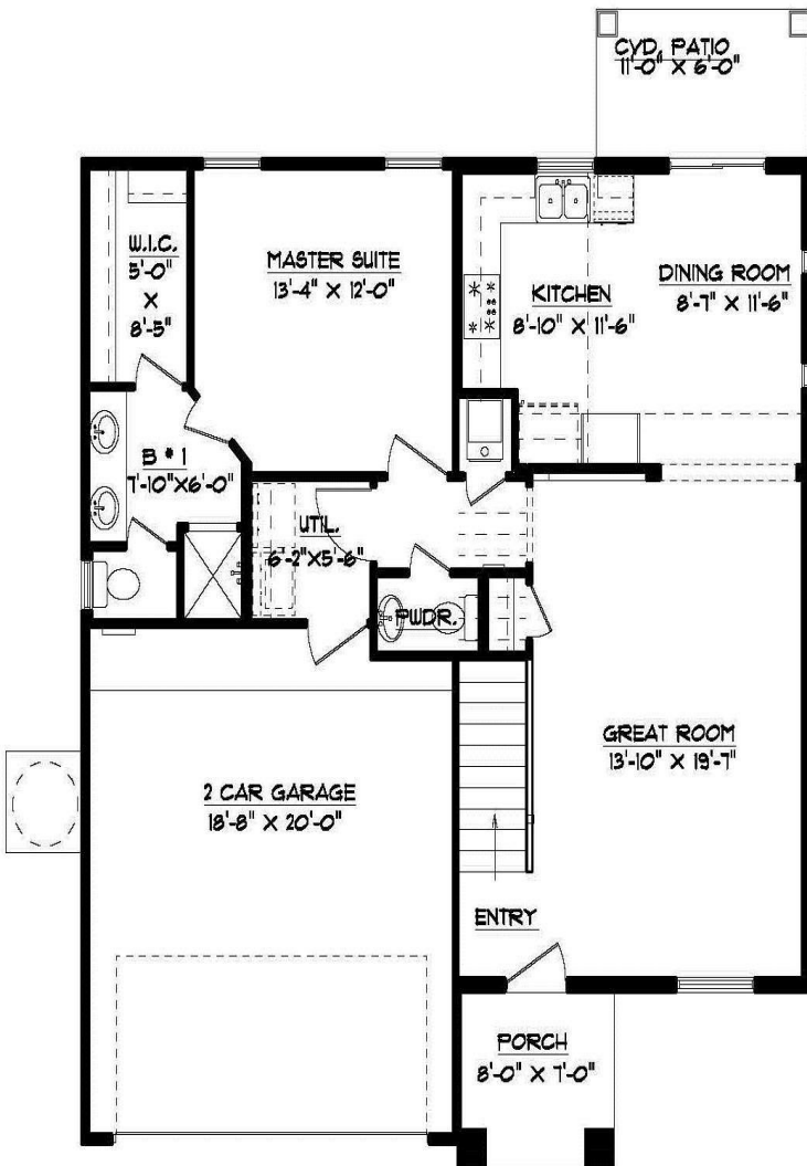
" FIRST FLOOR PLAN " W 37'-4" X D 38'-8"
