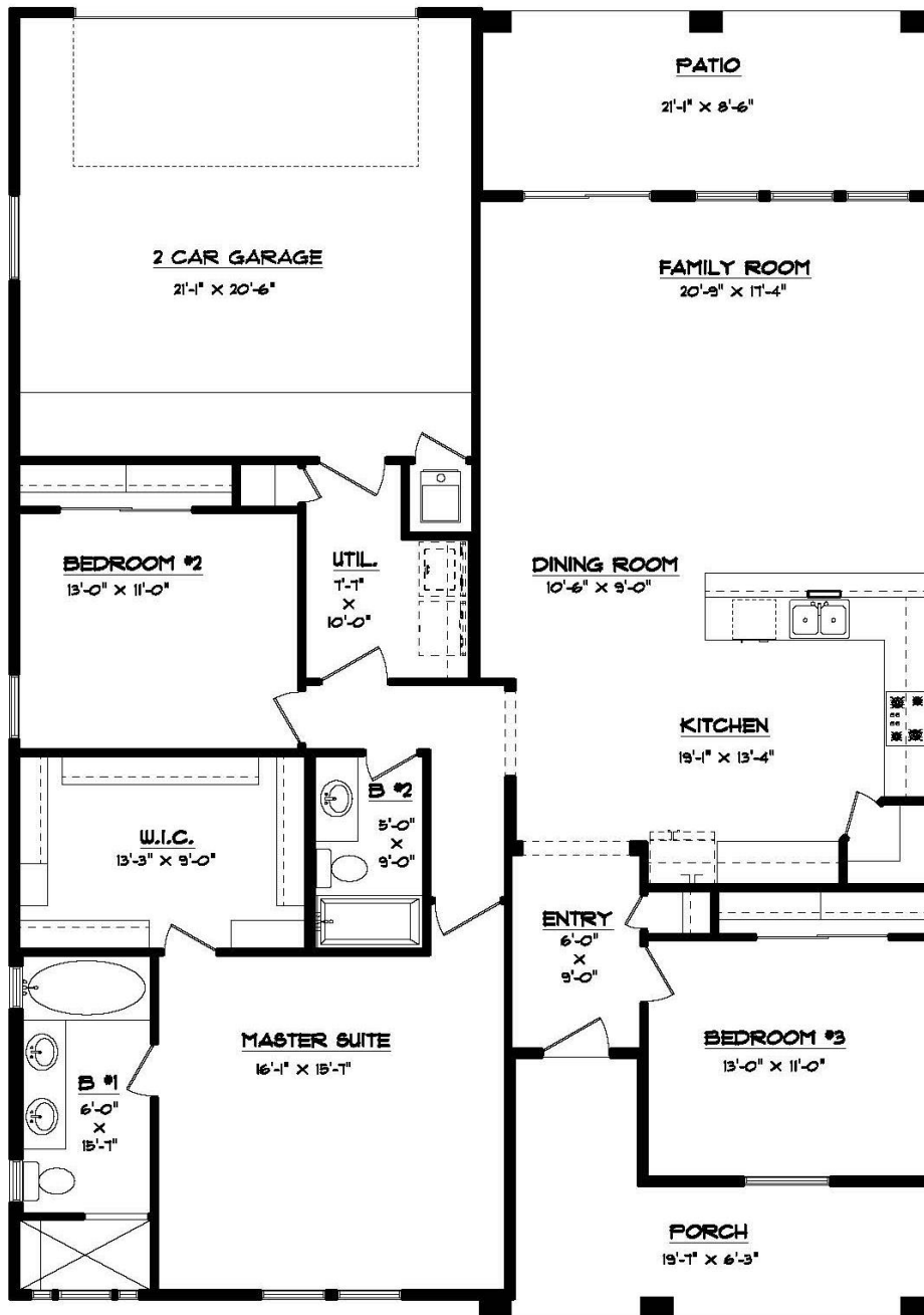
FLOOR PLAN 42'-9" X 59'-10"
