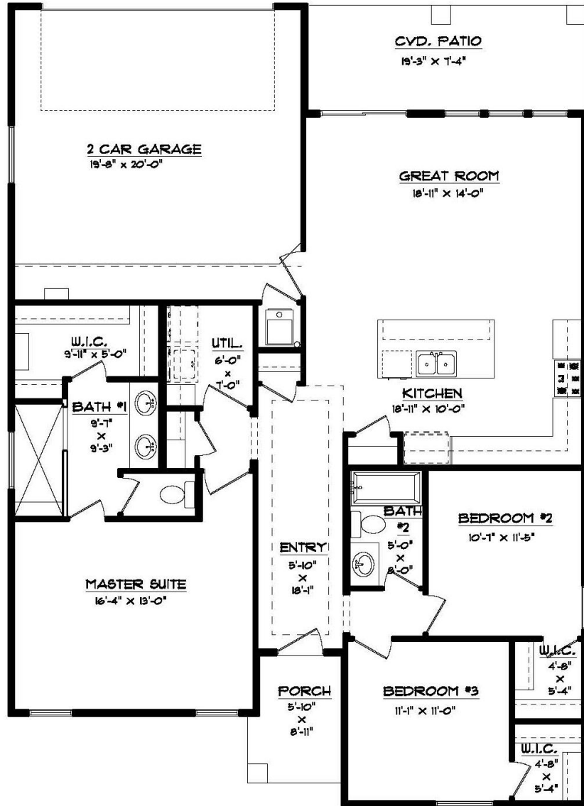
FLOOR PLAN 39'-6" X 55'-0"
