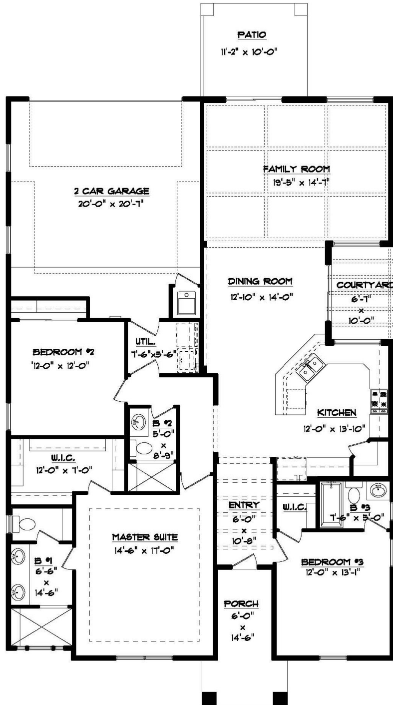
FLOOR PLAN 40'-6" x 58'-11 1/2"
